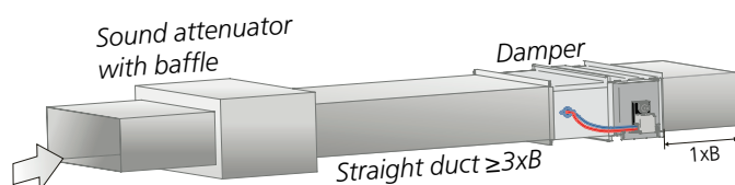
Figure 10. Straight duct section requirements 3 \times B in case of sound attenuator with baffle. Applies to both supply and extract air.
